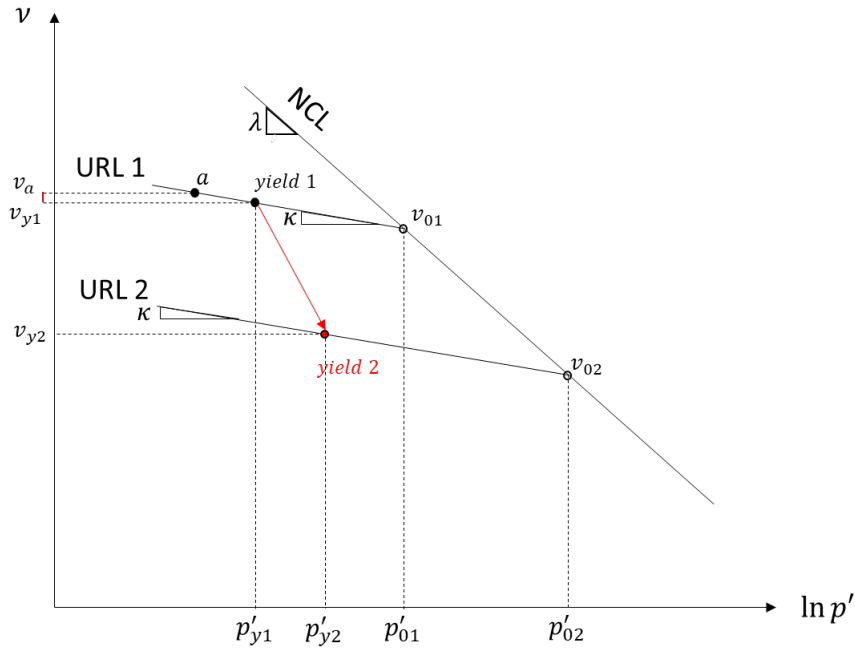
Figure B. Global stress path in the ( v - \ln(p') ) plane. The path tackled in question 2 is the one from the point yield 1 to the point yield 2.
