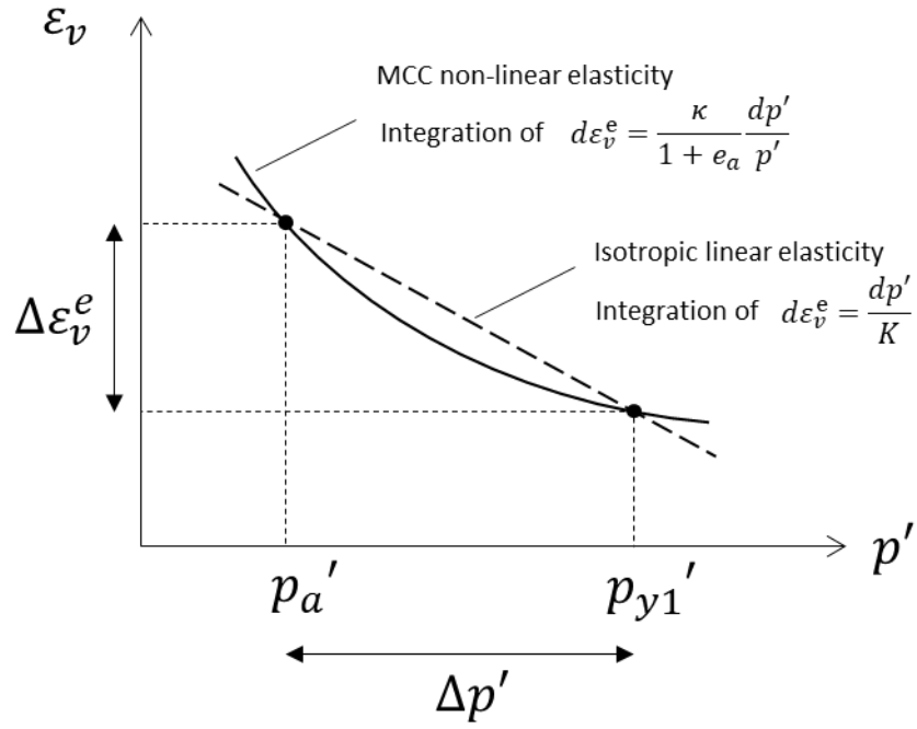
Figure F. Schematic representation of the estimation of the bulk modulus K for the computation of the shear modulus G .
